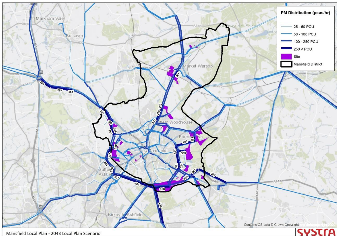
Figure 5. Development Distribution Local Plan Scenario – PM
