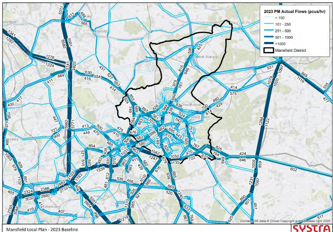
Figure 4. Highway Flows 2023 Baseline – PM
