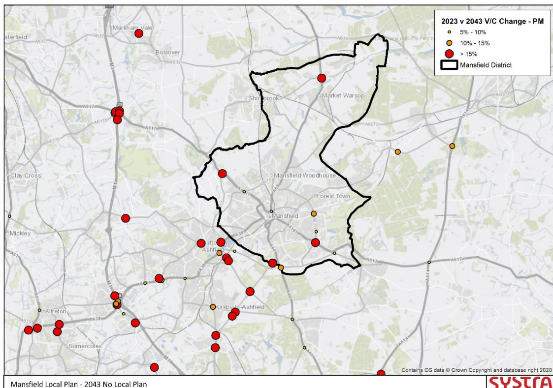
Figure 10. Change in Junction Congestion 2023 Baseline v 2043 No Local Plan - PM
