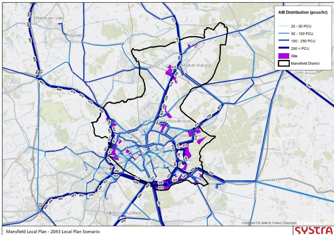
Figure 4. Development Distribution Local Plan Scenario – AM
