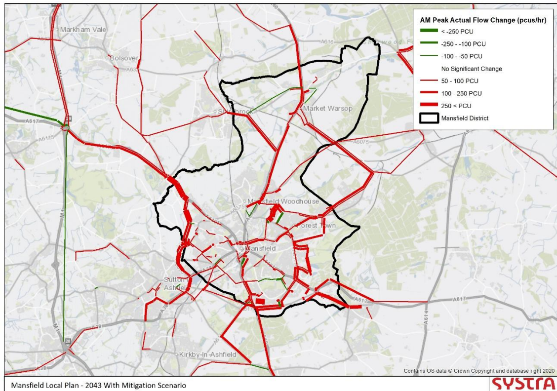
Figure 17. Highway Flow Change 2043 With Mitigation Scenario vs No Local Plan Scenario – AM
