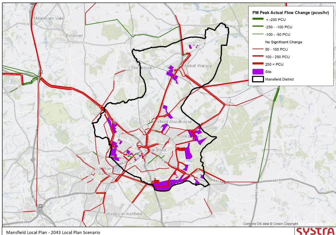
Figure 7. Highway Flow Change 2043 No Local Plan vs Local Plan Scenario – PM
