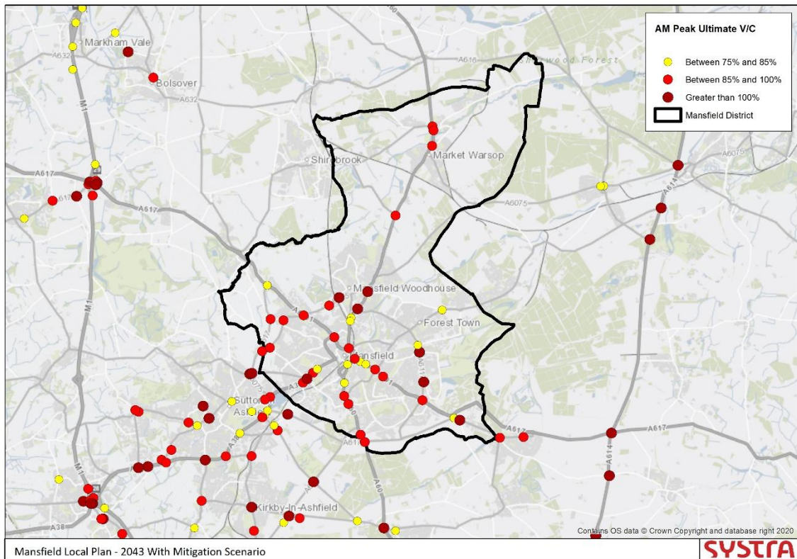
Figure 23. Junction Congestion 2043 With Mitigation Scenario – AM
