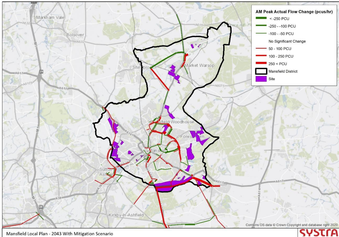
Figure 15. Highway Flow Change 2043 With Mitigation Scenario vs Local Plan Scenario – AM
